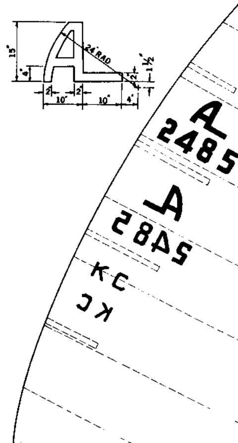
OFFICIAL LAYOUT OF SAIL INSIGNIA & NUMBERS
